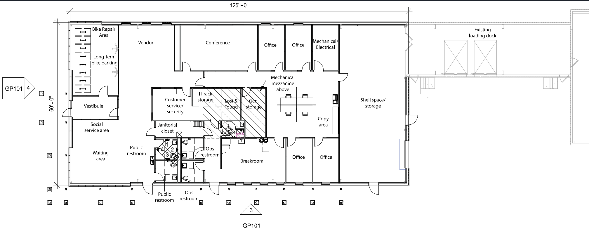
1 FLOOR PLAN
